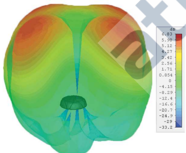
Typical 3D Pattern (2600MHz)
