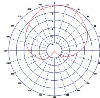
Typical E-Plane Pattern GPS/GNSS
