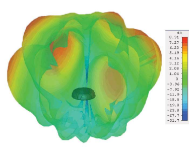
Typical 3D Pattern WiFi (5400MHz)
