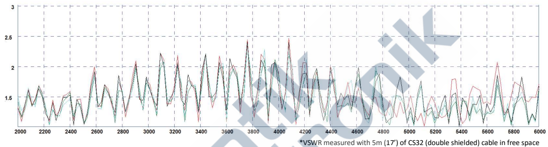
Typical Isolation -CELL/LTE - Elements 1-4
