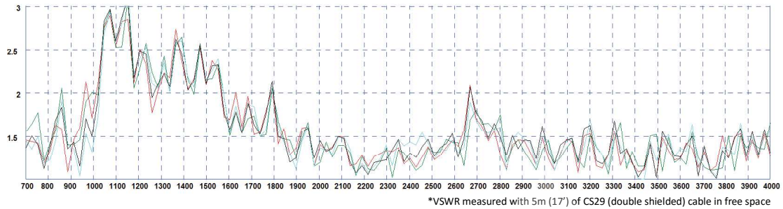
Typical VSWR - WiFi - Elements 1-4
