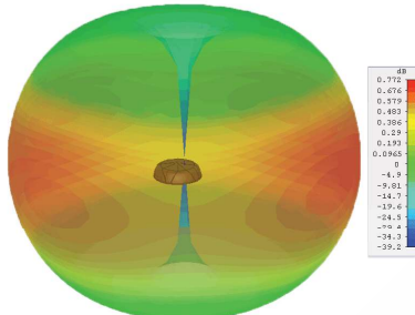
Typical 3D Pattern (1900MHz)
