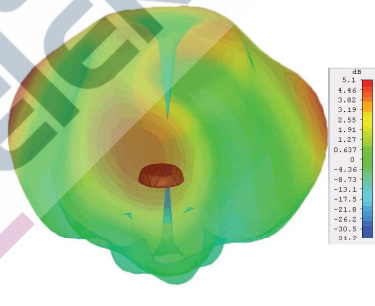
Typical 3D Pattern (3600MHz)
