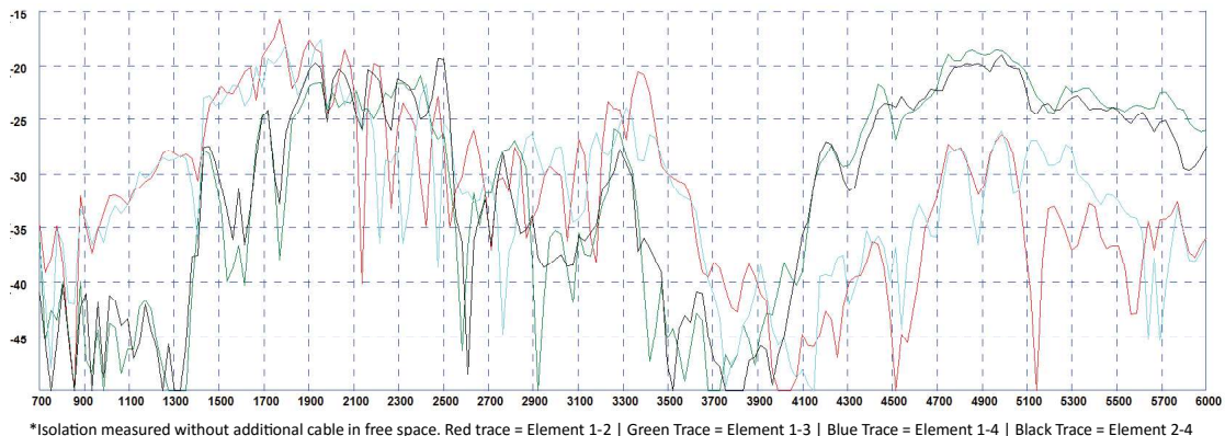
Typical Isolation -WiFi - Elements 1-4
