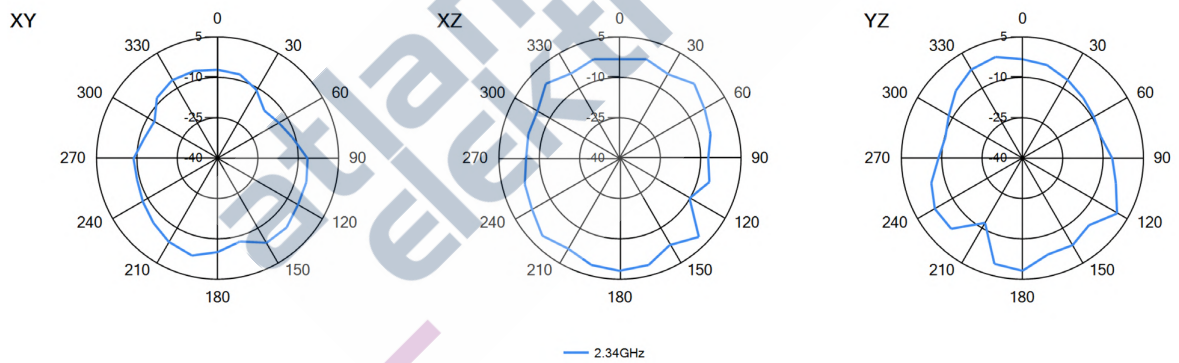
3D pattern at 2340MHz
