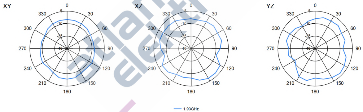
3D pattern at 1930MHz
